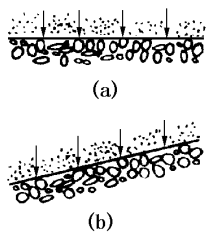
图B.0.3-1 I型反滤
